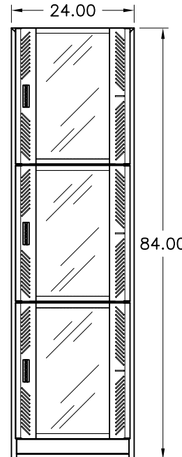
FRONT VIEW
