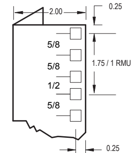
M6 CAGE-NUT RAIL
