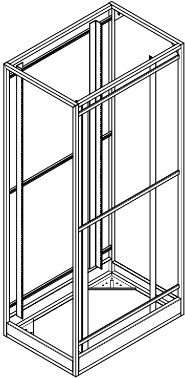
ISOMETRIC VIEW
