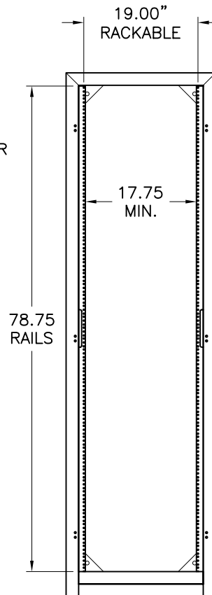
FRONT VIEW
