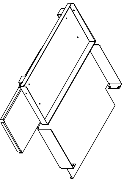
ISOMETRIC VIEW KEYBOARD TRAY AND MOUSE PAD SHOWN IN EXTENDED POSITION
